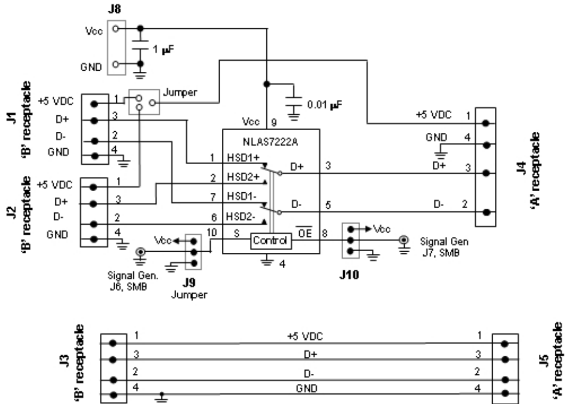
Figure 7. Schematic of the NLA7222A USB Demo Board
