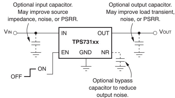
Figure 31. Typical Application Circuit for Fixed-Voltage Versions
