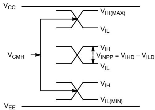
Figure 13. V_{CMR} Diagram
