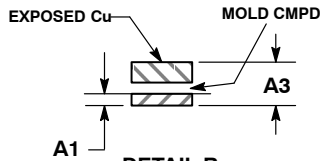
DETAIL B OPTIONAL CONSTRUCTION
