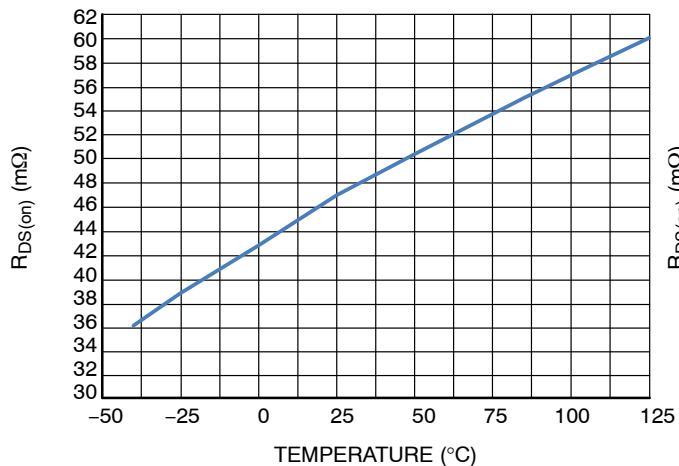
Figure 6. R_{DS(on)} ( m\Omega ) vs. Temperature ( ^{\circ}C ) at 3.3 V, I_{LOAD} 100 mA
