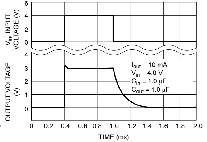
Figure 11. Turn-on Response
