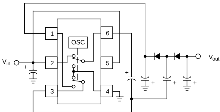
Figure 22. Negative Output Voltage Doubler
