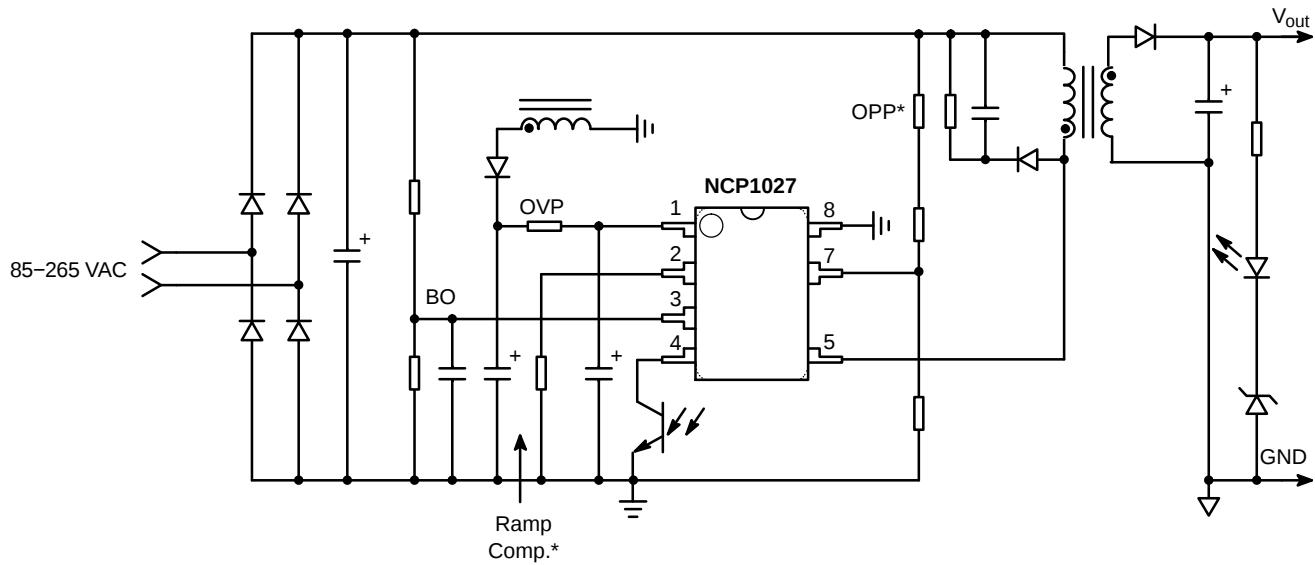
Figure 1. Typical Application
